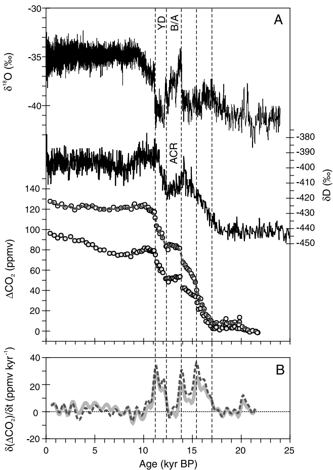
18. Ice core records showing CO 2 in phase with Antarctic warming. A) \delta^{18}\text{O} and \delta\text{D} = temperature records, \Delta\text{CO}_2 changing atmospheric carbon dioxide levels, higher curve taking into account coral reef and land vegetation changes since the last ice age. B) rate of change of carbon dioxide most of which occurs in three large pulses
